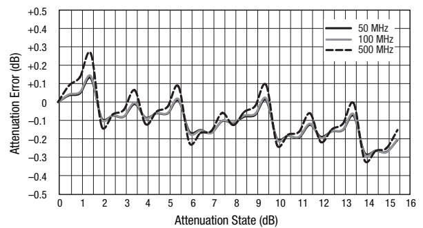
Figure 9. Attenuation Error vs Attenuation State (@ 50, 100, and 500 MHz)
