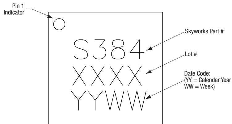
Figure 13. Typical Part Markings (Top View)
