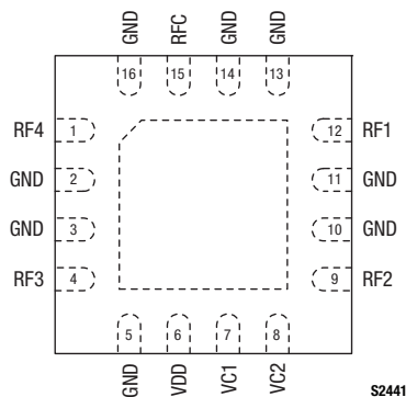
Figure 2. SKY13384-350LF Pinout (Top View)
