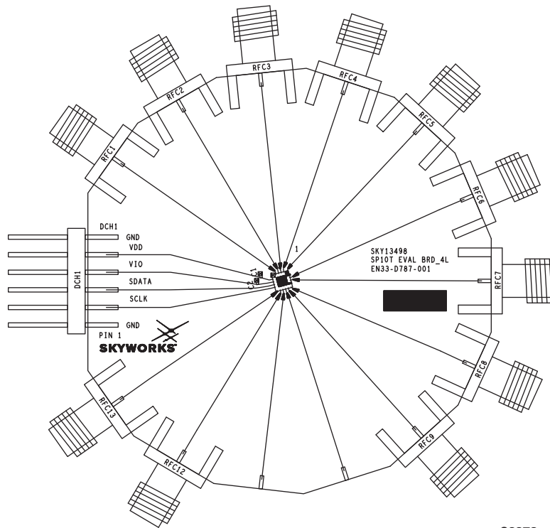
Figure 9. SKY13498-21 Evaluation Board Assembly Diagram
