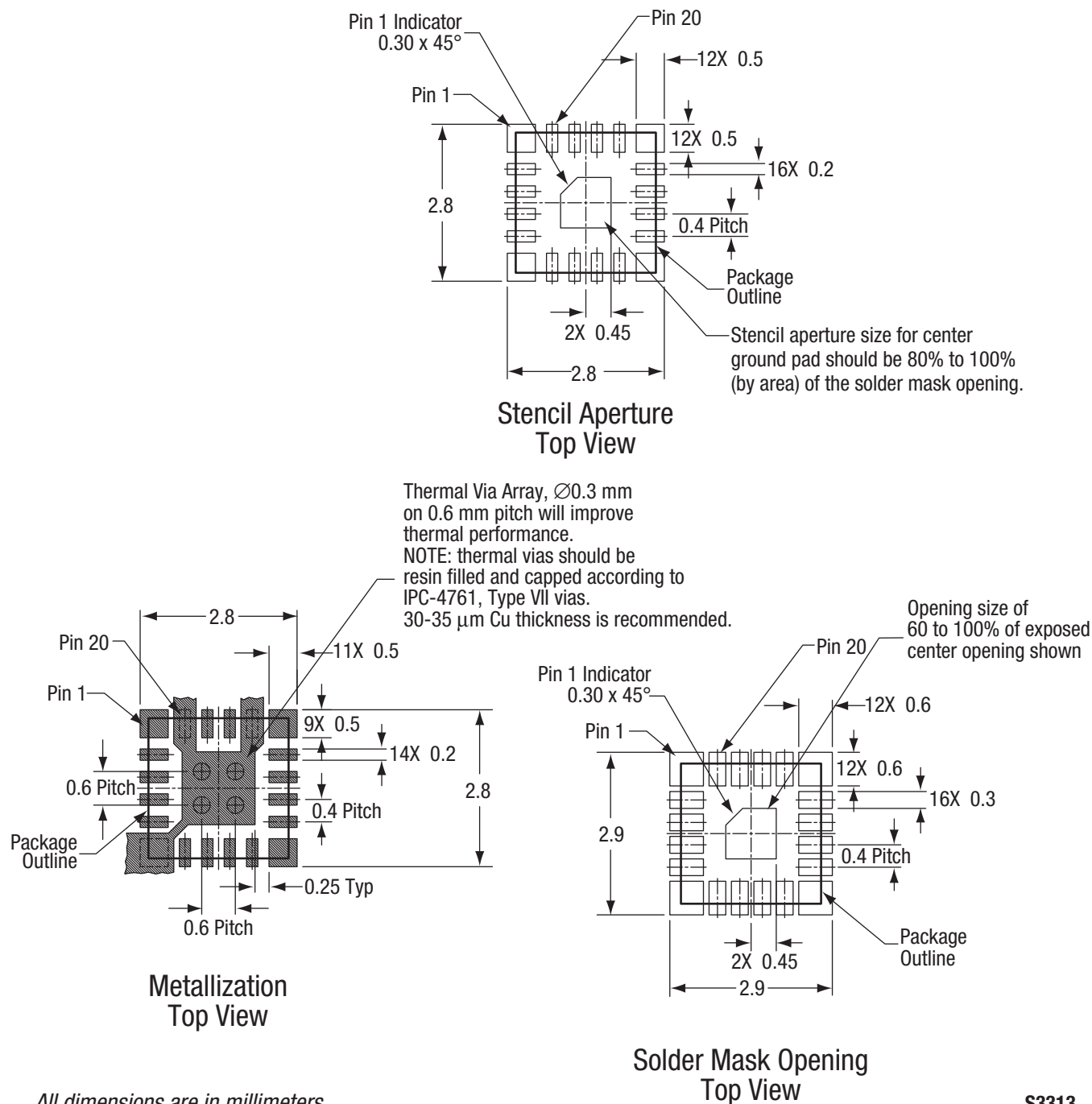
Figure 10. SKY13498-21 PCB Layout Footprint (Top View)
