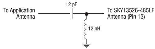
ESD Circuit 2
