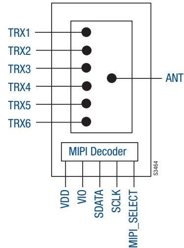
Figure 1. SKY13526-485LF Block Diagram
