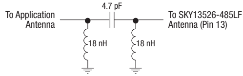
ESD Circuit 1
