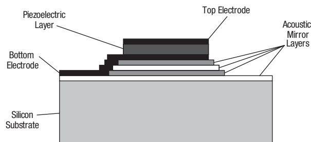
Simplified BAW Resonator Cross Section
