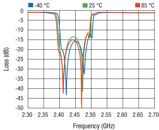
Return Loss Over Temperature – Wideband
