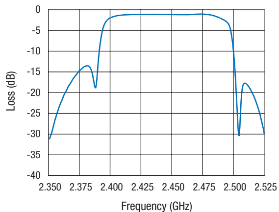
Insertion Loss – Narrowband
