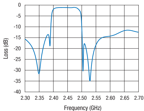
Insertion Loss – Wideband
