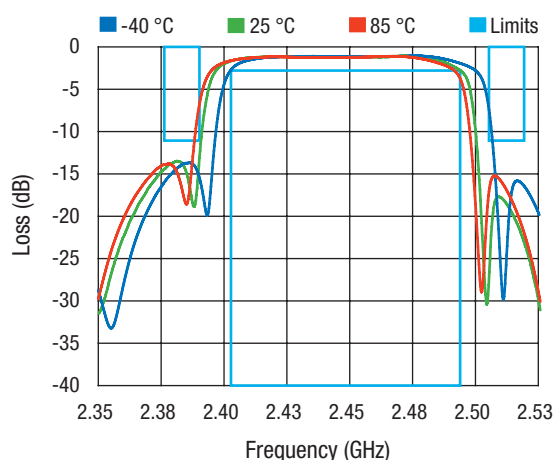
Insertion Loss Over Temperature – Narrowband
