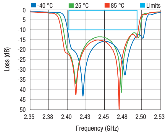
Return Loss Over Temperature – Narrowband
