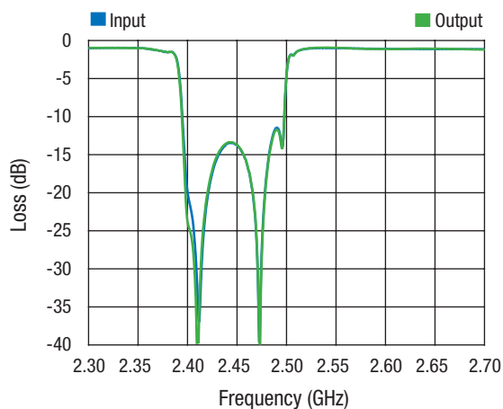
Return Loss – Wideband
