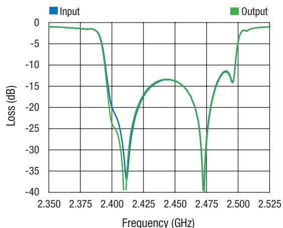
Return Loss – Narrowband
