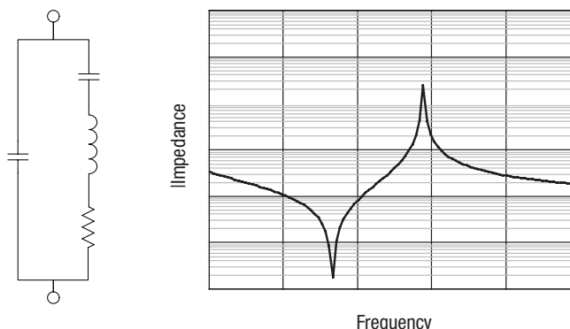
BAW Resonator Equivalent Circuit and Impedance vs. Frequency
