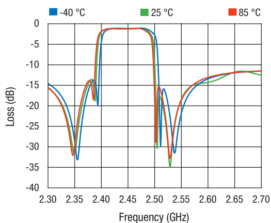
Insertion Loss Over Temperature – Wideband
