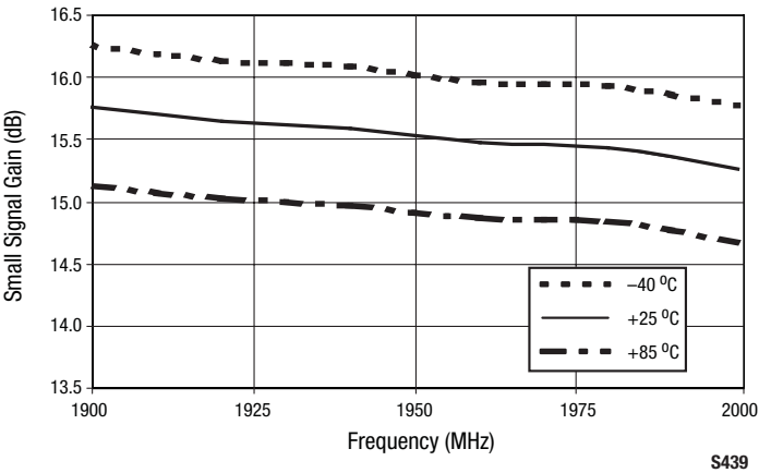
Figure 5. Typical Small Signal Gain From 1900 to 2000 MHz Over Temperature
