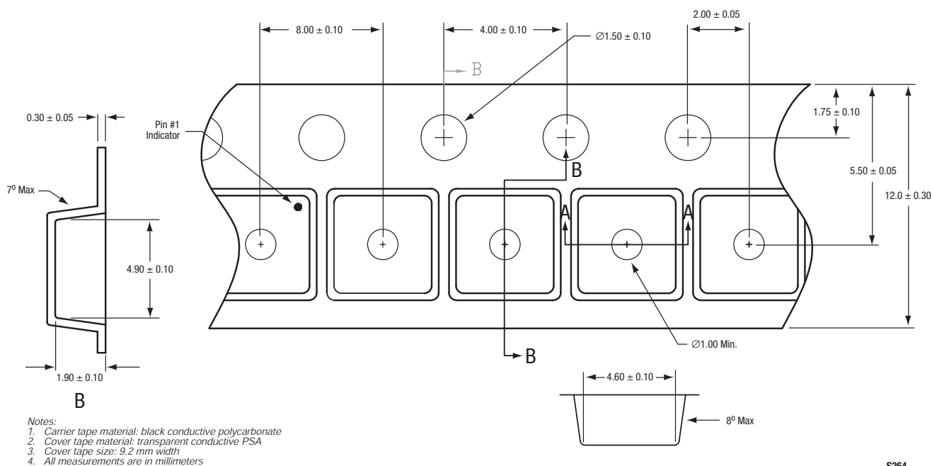
Figure 18. SKY65004-11 (4-Pin SOT-89) Tape and Reel Dimensions
