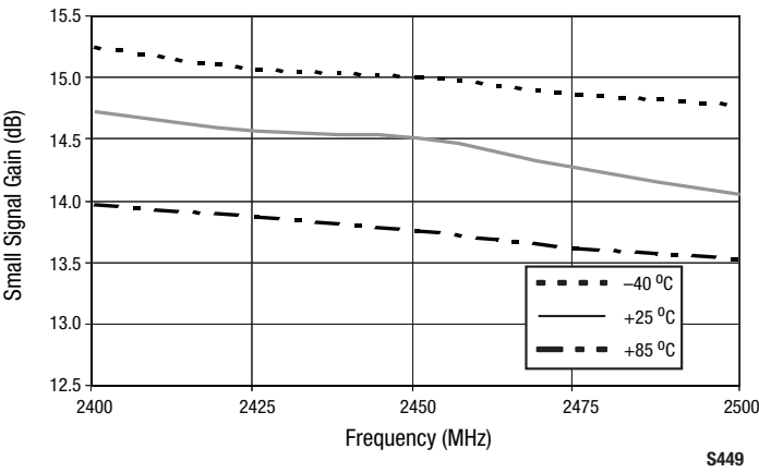
Figure 7. Typical Small Signal Gain From 2400 to 2500 MHz Over Temperature
