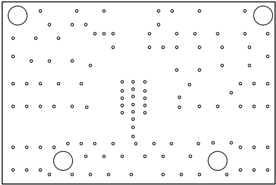
Layer 3: Ground
