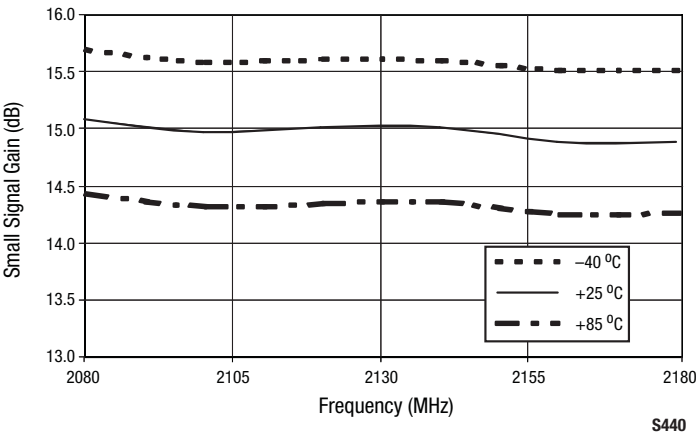
Figure 6. Typical Small Signal Gain From 2080 to 2180 MHz Over Temperature
