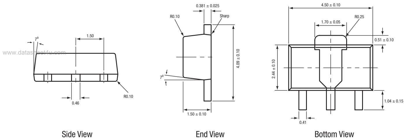
Figure 17. SKY65004-11 (4-Pin SOT-89) Package Dimensions
