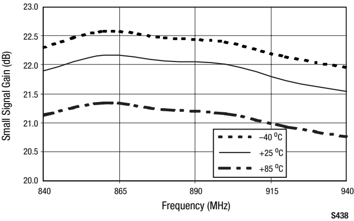
Figure 4. Typical Small Signal Gain From 840 to 940 MHz Over Temperature
