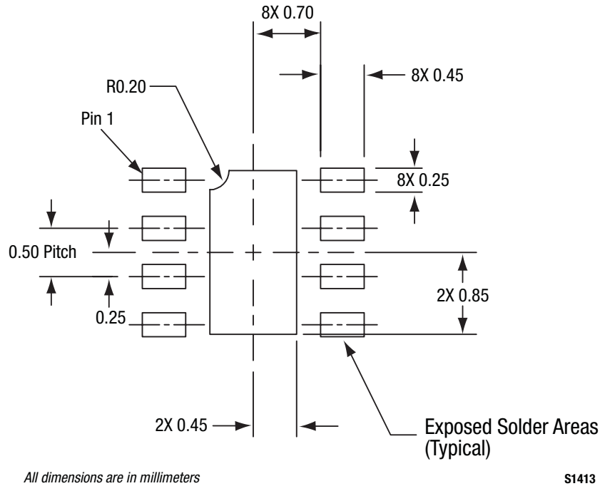
Figure 12. SKY65037-360LF PCB Layout Footprint
