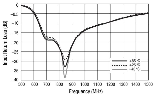
Figure 5. Input Return Loss vs Frequency Over Temperature, P_{IN} = -20\text{ dBm}
