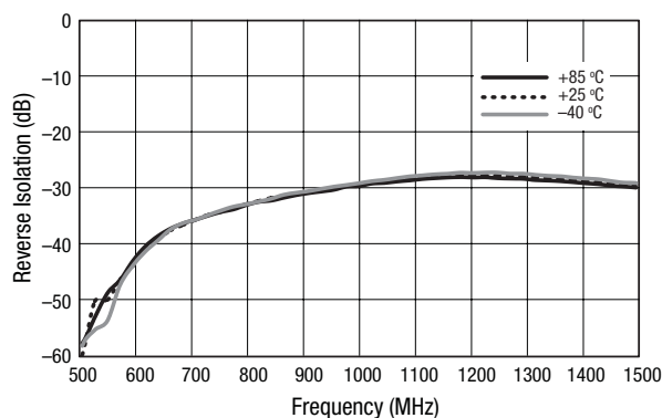
Figure 7. Reverse Isolation vs Frequency Over Temperature, P_{IN} = -20\text{ dBm}
