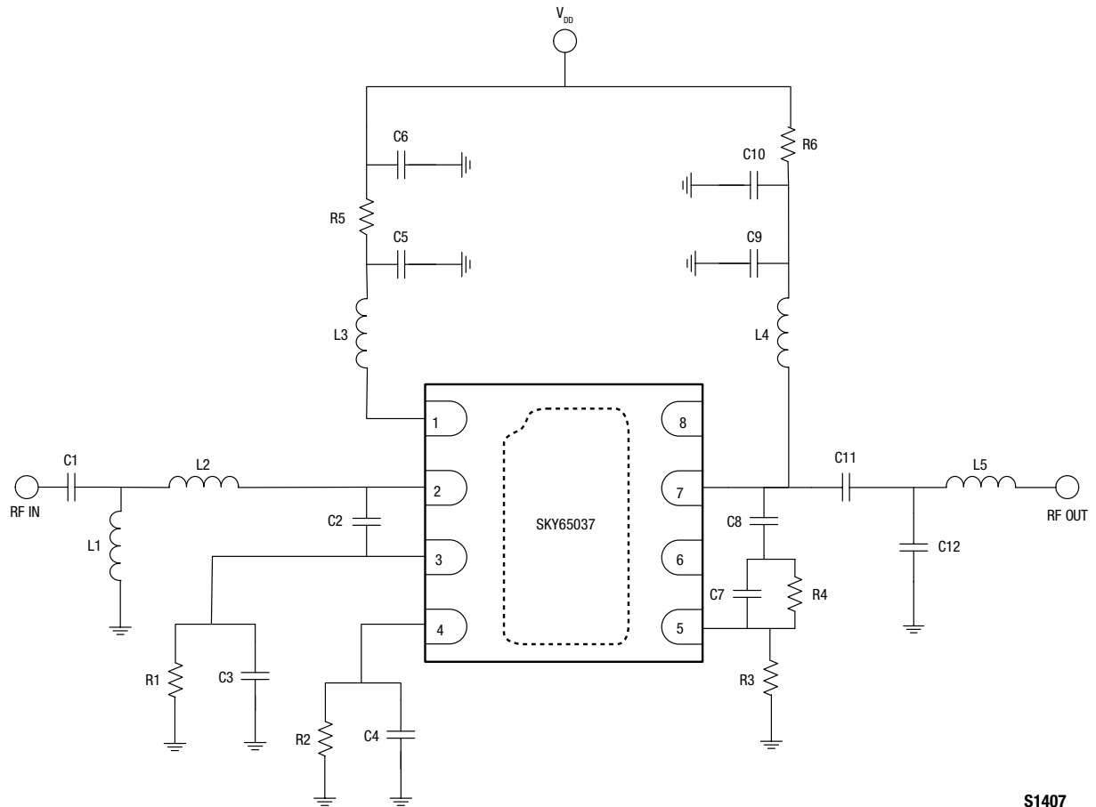
Figure 11. SKY65037-360LF Evaluation Board Schematic
