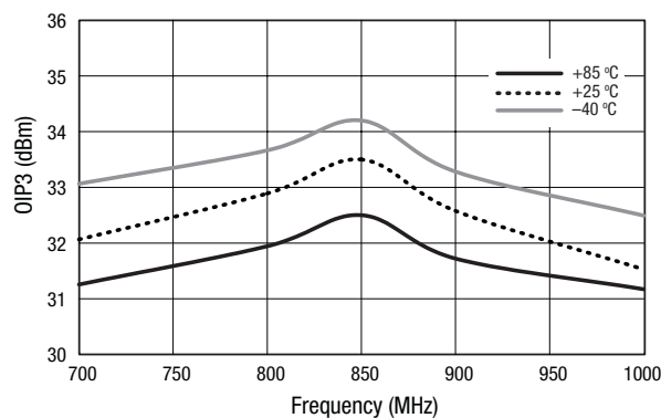
Figure 8. OIP3 vs Frequency Over Temperature, P_{IN} = -18\text{ dBm/Tone} , 5 MHz Tone Spacing
