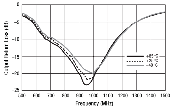
Figure 4. Output Return Loss vs Frequency Over Temperature, P_{IN} = -20\text{ dBm}
