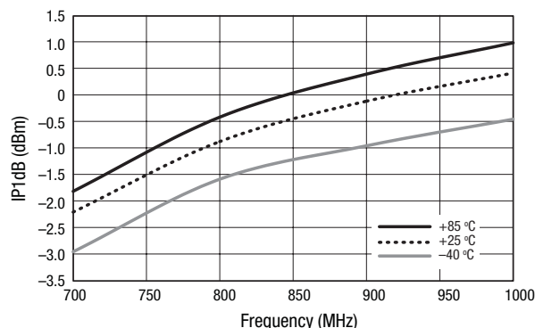
Figure 9. IP1dB vs Frequency Over Temperature
