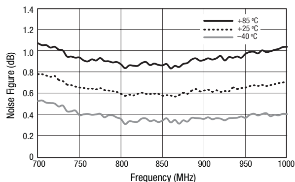
Figure 6. Noise Figure vs Frequency Over Temperature, Input RF Connector and Board Trace De-Embedded From Measurement
