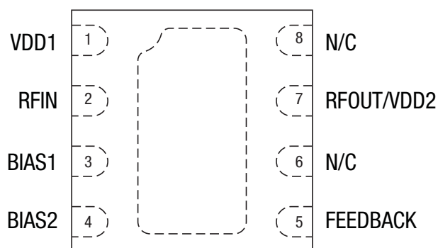
Figure 2. SKY65037-360LF Pinout – 8-Pin QFN (Top View)
