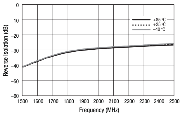
Figure 12. Reverse Isolation vs Frequency Over Temperature, P_{IN} = -20\ \text{dBm}
