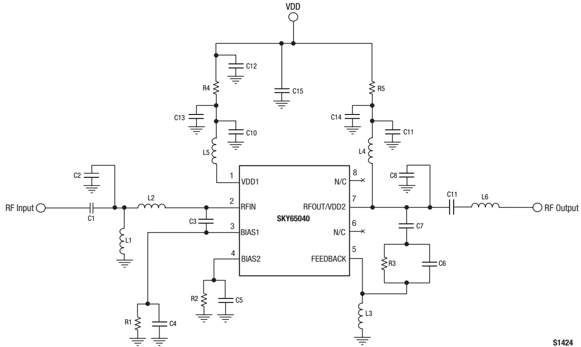
Figure 20. SKY65040-360LF Evaluation Board Schematic Diagram (Feedback Circuit)
