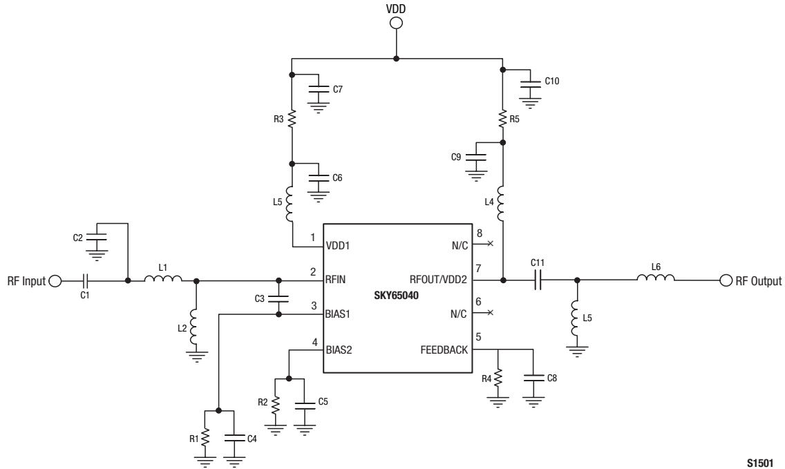
Figure 18. SKY65040-360LF Evaluation Board Schematic Diagram (High Gain Circuit)
