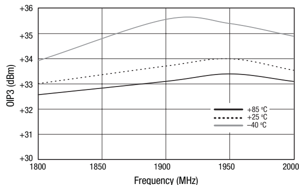
Figure 15. OIP3 vs Frequency Over Temperature, P_{IN} = -18\ \text{dBm/Tone} , 5 MHz Tone Spacing
