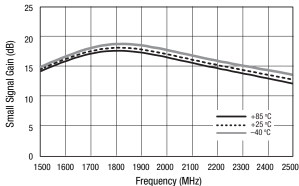
Figure 10. Small Signal Gain vs Frequency Over Temperature, P_{IN} = -20\ \text{dBm}
