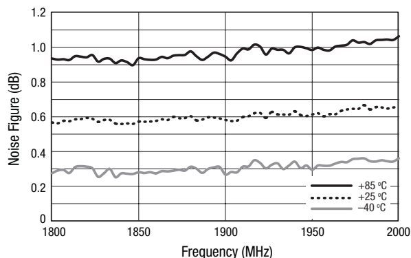
Figure 14. Noise Figure vs Frequency Over Temperature, Input RF Connector and Board Trace De-Embedded From Measurement
