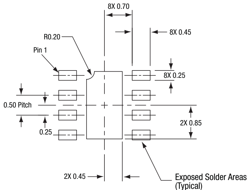
Figure 21. SKY65040-360LF PCB Layout Footprint
