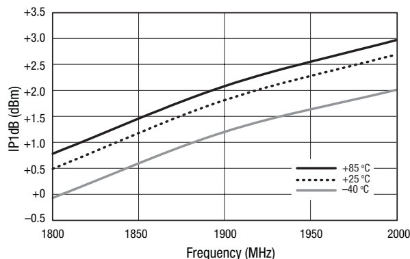
Figure 16. IP1dB vs Frequency Over Temperature
