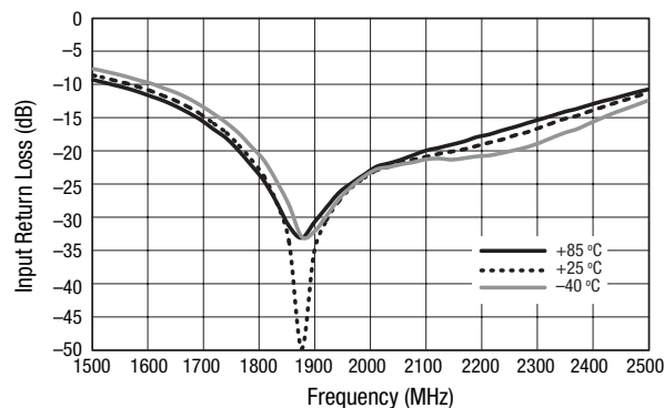
Figure 11. Input Return Loss vs Frequency Over Temperature, P_{IN} = -20\ \text{dBm}
