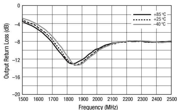
Figure 13. Output Return Loss vs Frequency Over Temperatures, P_{IN} = -20\ \text{dBm}
