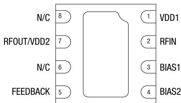
Figure 2. SKY65040-360LF Pinout – 8-Pin QFN (Bottom View)
