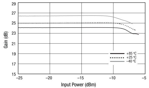
Figure 9. Gain vs Input Power Over Temperature, f = 1950 MHz
