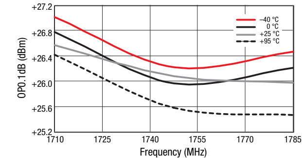
Figure 24. OP0.1dB vs Frequency Over Temperature
