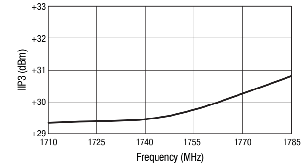
Figure 20. IIP3 vs Frequency ( P_{IN} = -10 dBm)
