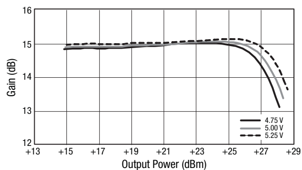
Figure 34. Gain vs Output Power Over Voltage
