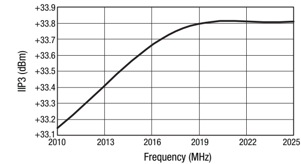
Figure 62. IIP3 vs Frequency ( P_{IN} = -10 dBm)
