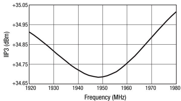
Figure 51. IIP3 vs Frequency ( P_{IN} = -10 dBm)
