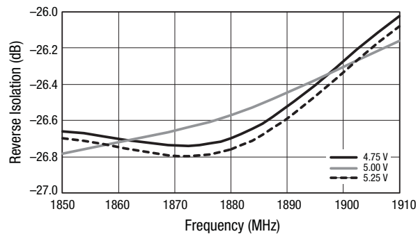
Figure 32. Reverse Isolation vs Frequency Over Voltage
