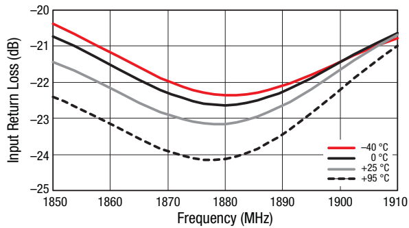
Figure 25. Input Return Loss vs Frequency Over Temperature
