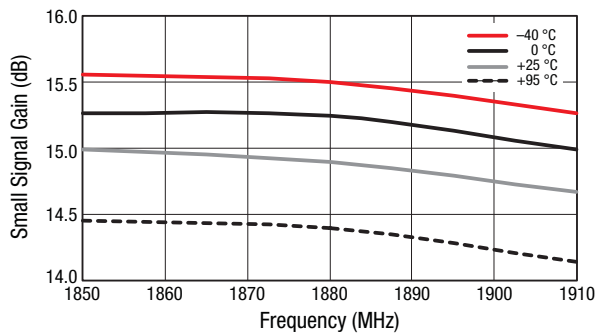
Figure 29. Small Signal Gain vs Frequency Over Temperature
