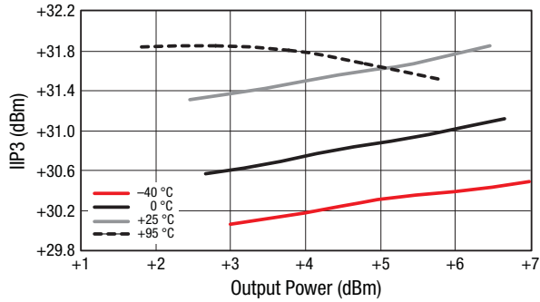
Figure 37. IIP3 vs Output Power Over Temperature
