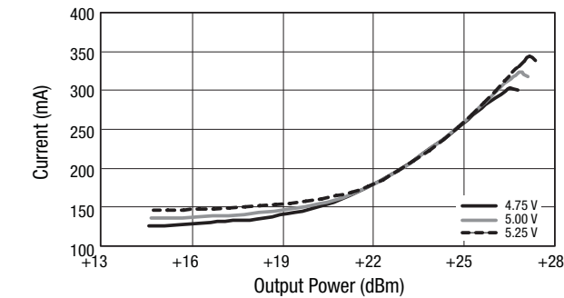
Figure 64. Operational Current vs Output Power Over Voltage
