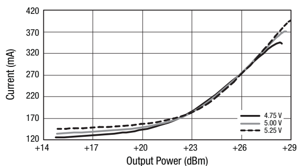
Figure 53. Operational Current vs Output Power Over Voltage
