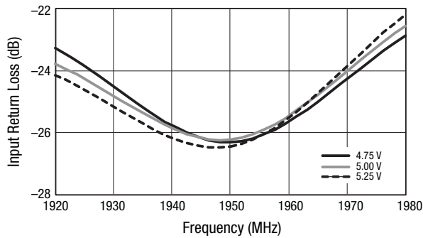
Figure 45. Input Return Loss vs Frequency Over Voltage
