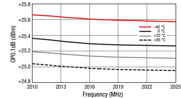
Figure 66. OP0.1dB vs Frequency Over Temperature
