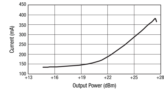
Figure 22. Operational Current vs Output Power
