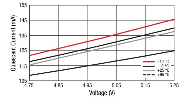
Figure 43. Quiescent Current vs Voltage Over Temperature
