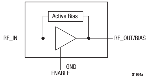
Figure 1. SKY65095-360LF Functional Block Diagram
