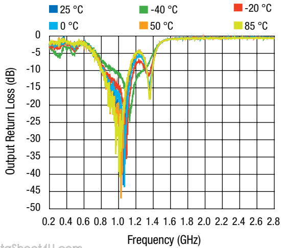
Output Return Loss vs. Frequency, V_{CC} = 3.5 V P_{IN} = -30 dBm, V_{APC1,2} = 2.7 V
