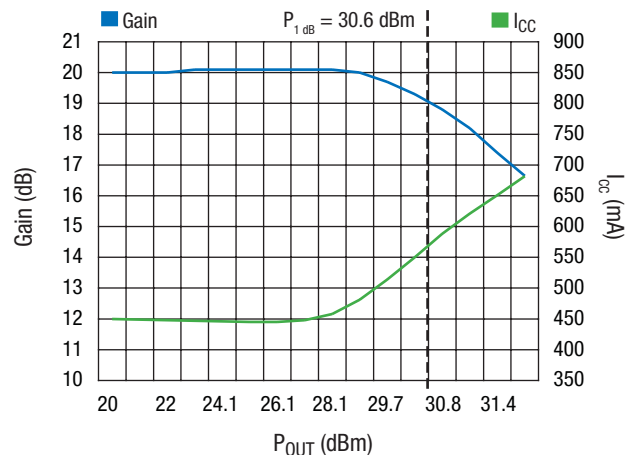
SKY65113 Gain, I_{CC} vs. P_{OUT}
