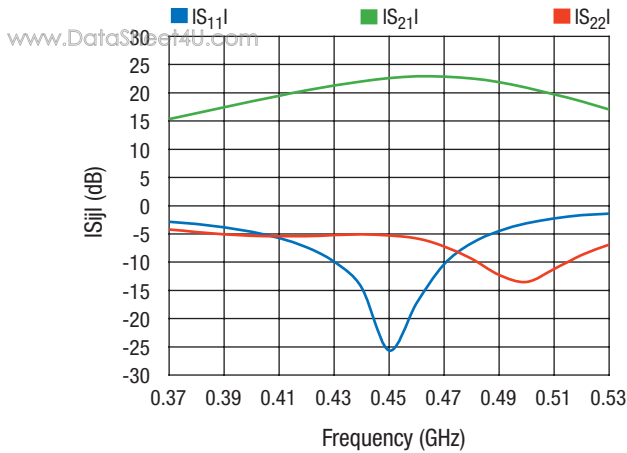
SKY65113 Tuned for 450 MHz
