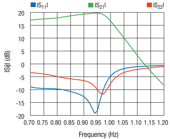
SKY65113 Tuned for 940 MHz
