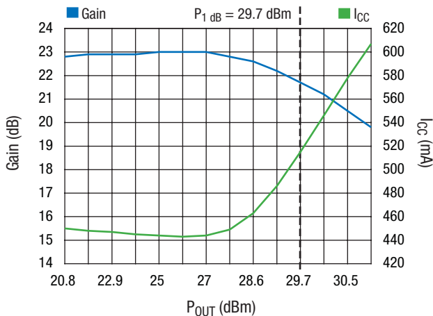
SKY65113 Gain, I_{CC} vs. P_{OUT}
