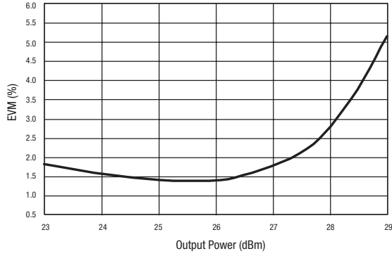
Figure 9. EVM vs P out for 802.11g
