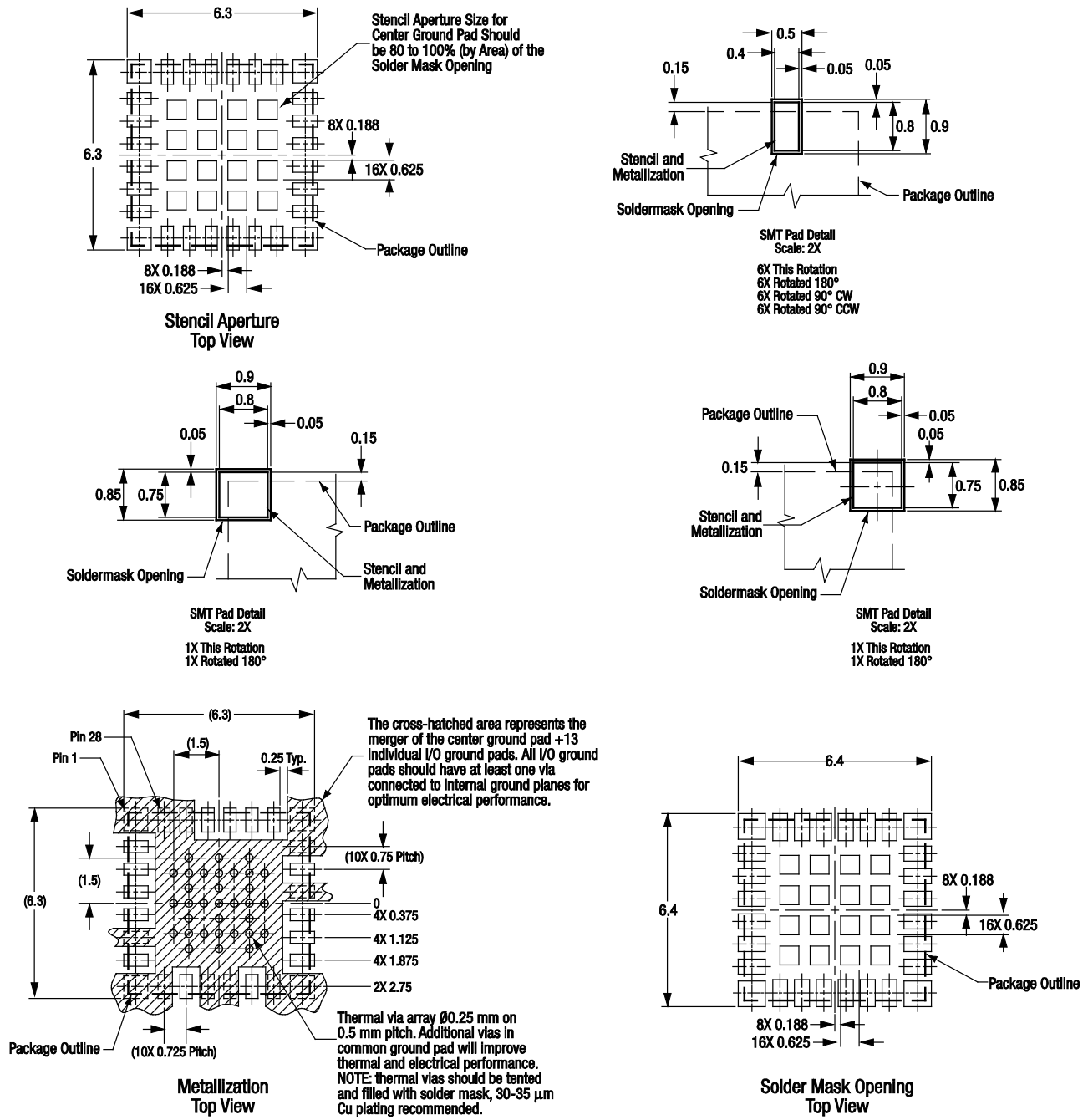
Figure 26. SKY65313-21 PCB Layout Footprint
