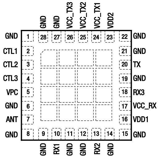
Figure 1. SKY65313-21 Pinout – 28-Pin MCM (Top View)
