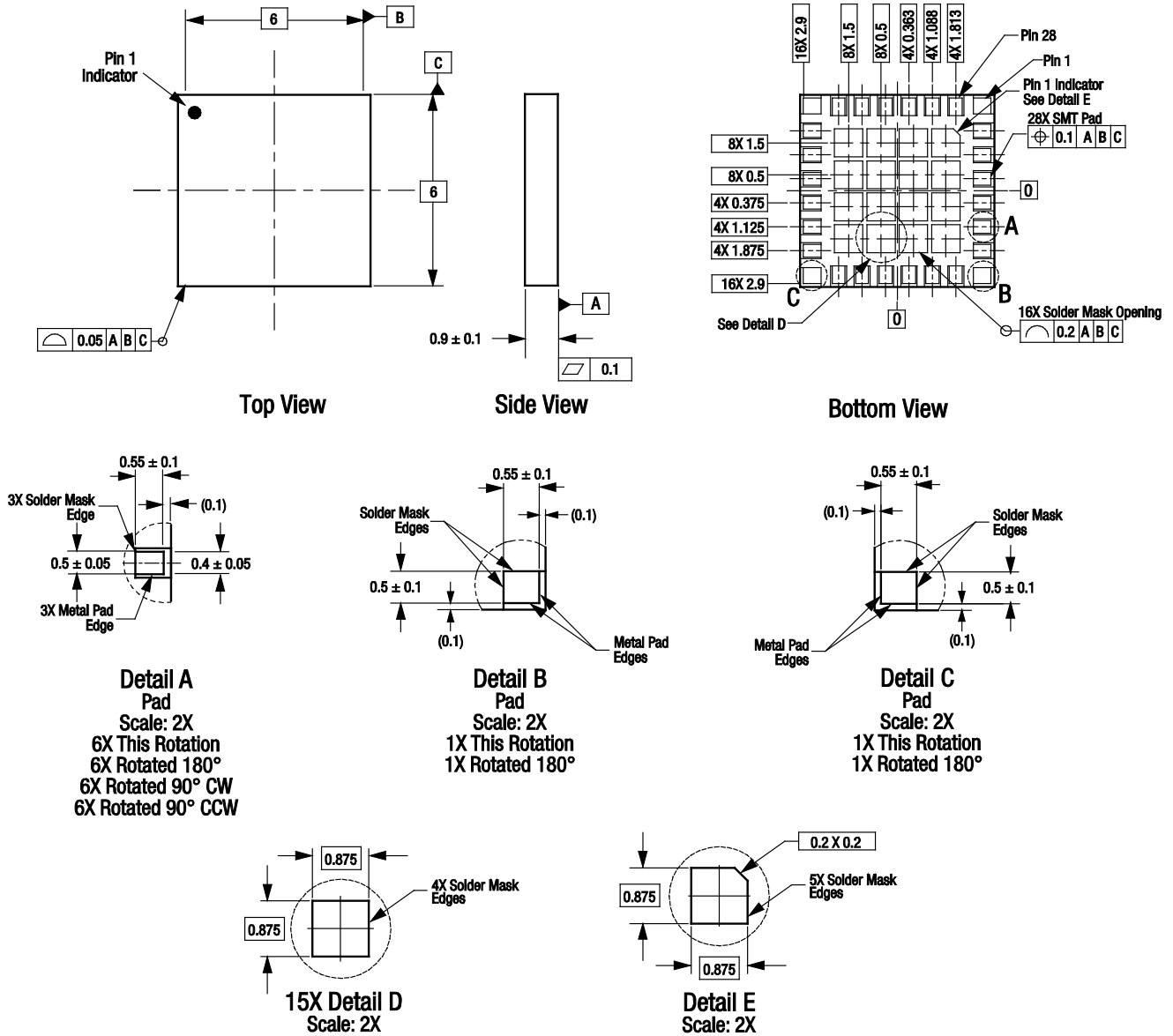
Figure 27. SKY65313-21 28-Pin MCM Package Dimensions
