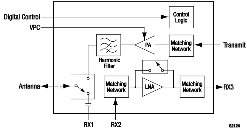
Figure 2. SKY65313-21 Block Diagram
