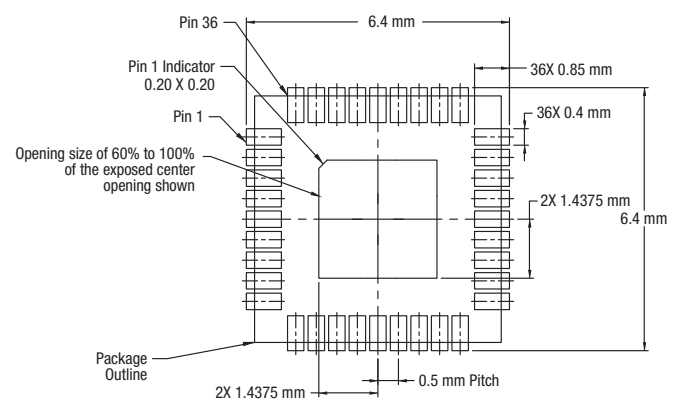
Solder Mask Opening
