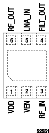
Figure 2. SKY65709-81 Pinout – 6-Pin MCM (Top View)
