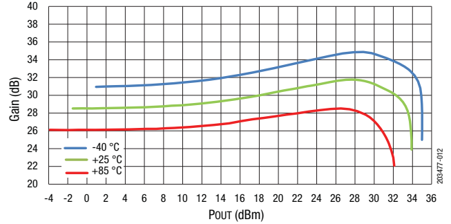
Figure 12. Gain vs Output Power @ 5787.5 MHz
