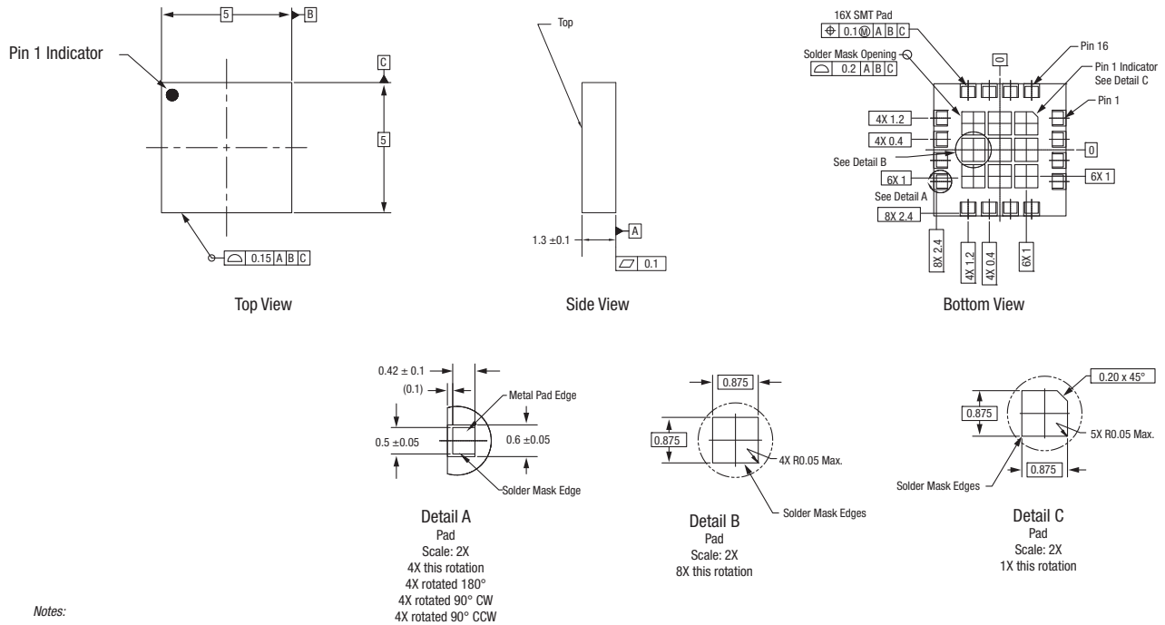
Figure 23. SKY66293-21 Package Dimensions
