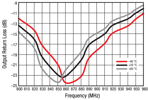
Figure 7. Small Signal Output Return Loss (S22) vs Frequency and Temperature, Narrow Band
