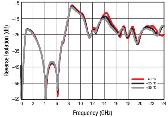
Figure 10. Small Signal Reverse Isolation (S12) vs Frequency and Temperature, Wide Band
