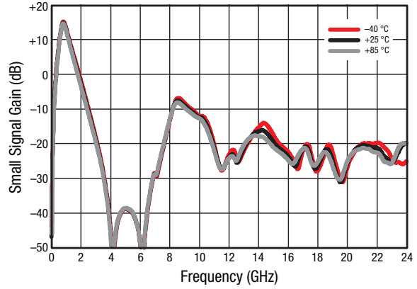
Figure 8. Small Signal Gain (S21) vs Frequency and Temperature, Wide Band
