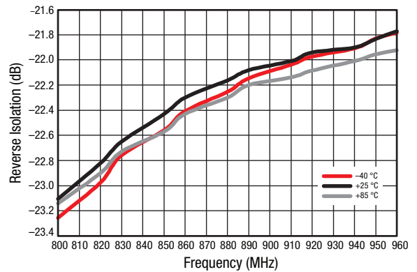
Figure 6. Small Signal Reverse Isolation (IS12) vs Frequency and Temperature, Narrow Band
