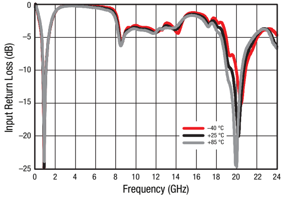
Figure 9. Small Signal Input Return Loss (S11) vs Frequency and Temperature, Wide Band
