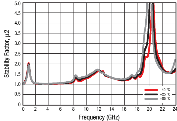
Figure 26. Stability Factor ( \mu^2 ) vs Frequency and Temperature, Wide Band
