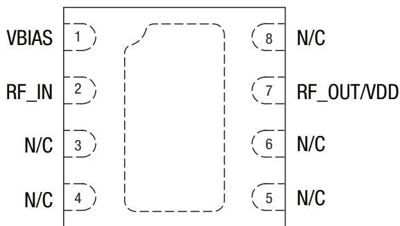
Figure 2. SKY67013-396LF Pinout – 8-Pin DFN (Top View)
