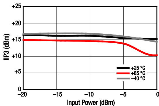
Figure 18. IIP3 vs Input Power Over Temperature @ 1200 MHz ( P_{IN} = -20 dBm, Tone Spacing = 1 MHz)
