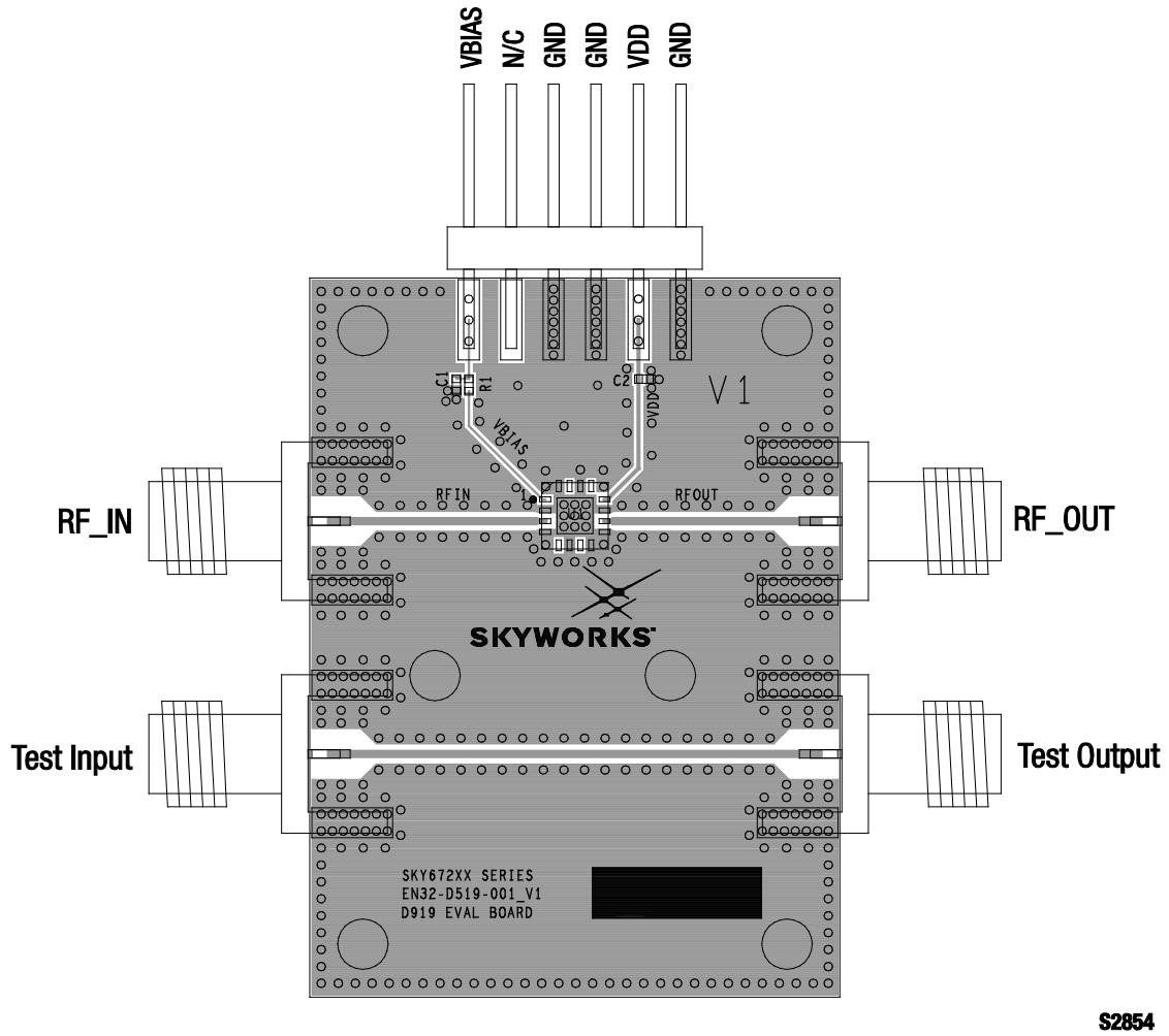
Figure 25. SKY67216-11 Evaluation Board Assembly Drawing
