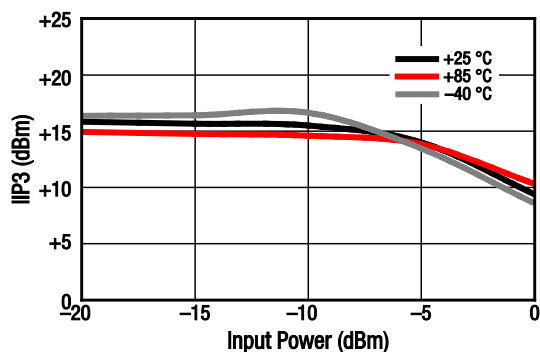
Figure 17. IIP3 vs Input Power Over Temperature @ 850 MHz ( P_{IN} = -20 dBm, Tone Spacing = 1 MHz)
