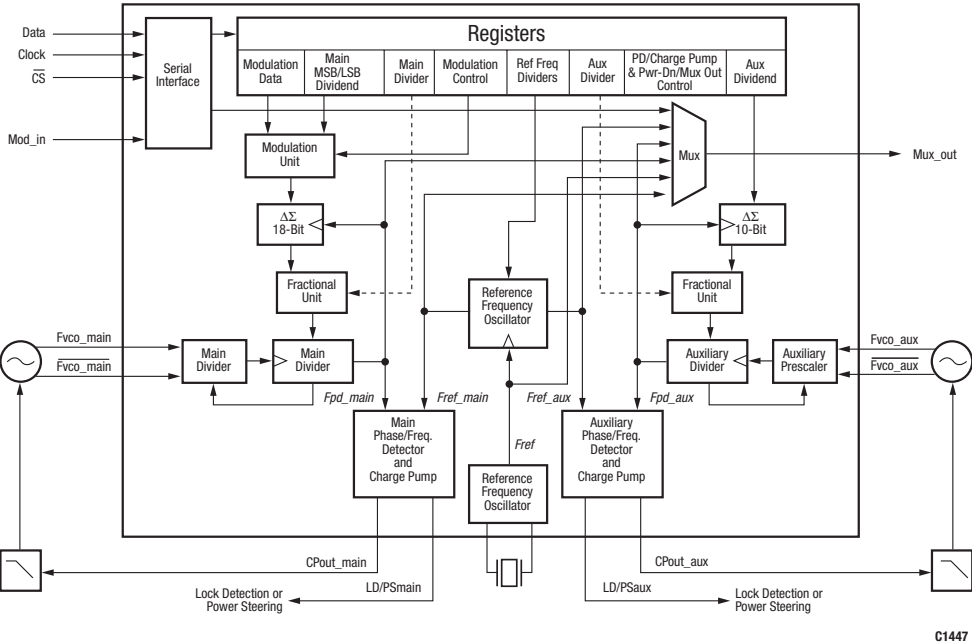
Figure 1. SKY72302 Functional Block Diagram
