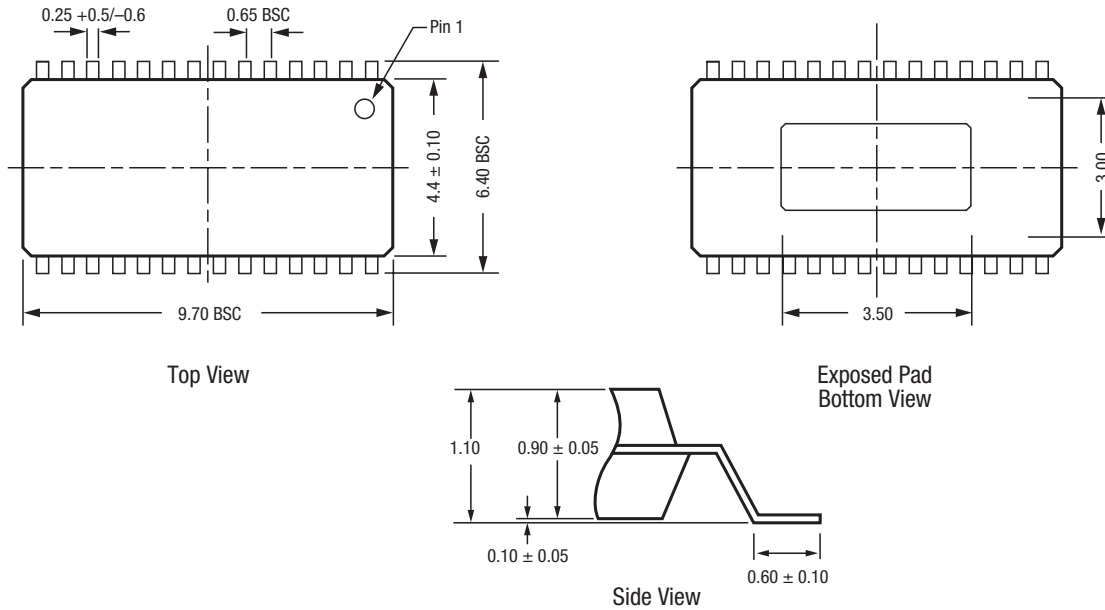
Figure 17. SKY72302 28-Pin EP-TSSOP Package Dimensions
