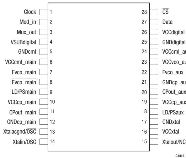
Figure 2. SKY72302 Pinout, 28-Pin EP-TSSOP (Top View)
