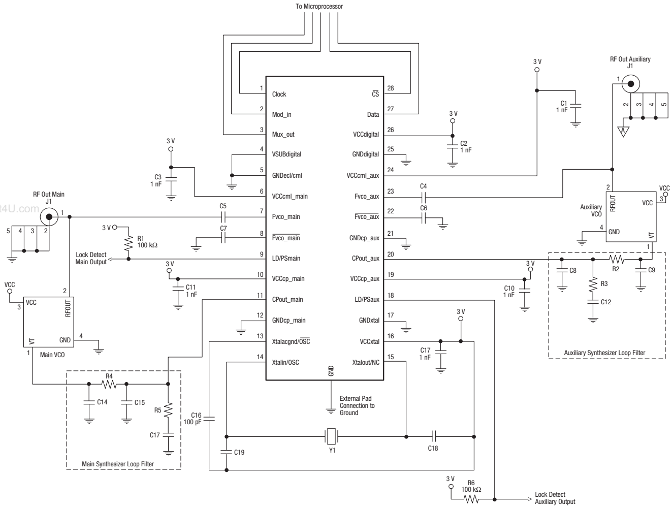
Figure 16. SKY72302 Application Schematic
