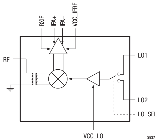
Figure 1. SKY73033-11 Block Diagram
