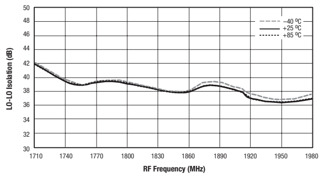
Figure 20. Mixer LO1 to LO2 Isolation vs Frequency and Temperature
