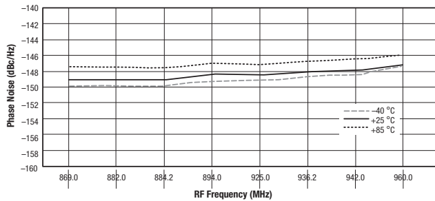
Figure 22. Phase Noise @ 800 kHz Offset vs Frequency and Temperature
