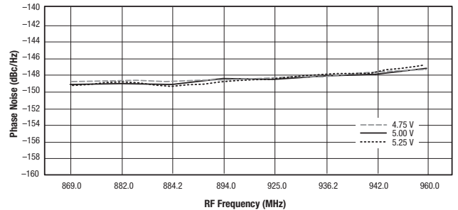
Figure 23. Phase Noise @ 800 kHz Offset vs Frequency and Supply Voltage
