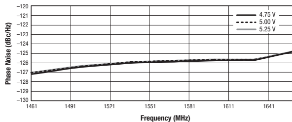
Figure 19. Phase Noise @ 200 kHz Offset vs Frequency and Supply Voltage
