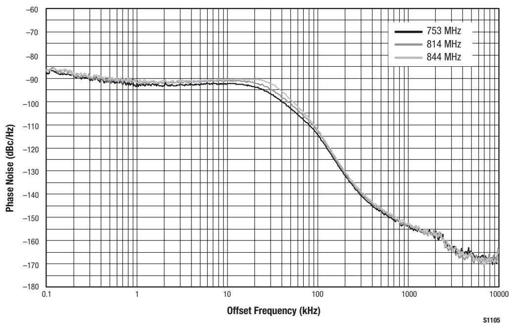
Figure 8. Single Sideband Phase Noise Measurements
