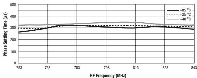
Figure 14. Phase Settling Time vs Frequency and Temperature
