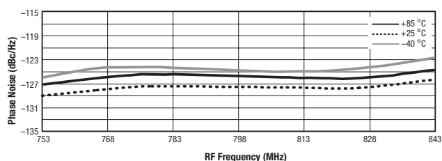
Figure 18. Phase Noise @ 200 kHz Offset vs Frequency and Temperature
