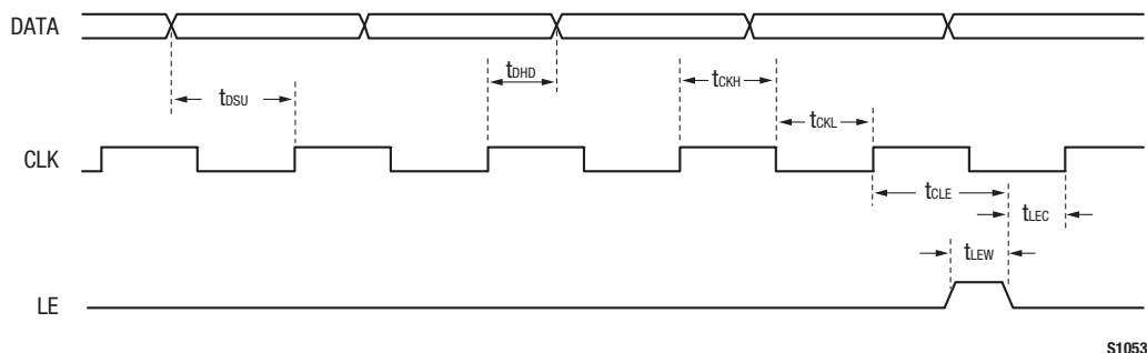
Figure 3. SKY73112-11 Serial Data Input Timing Diagram (MSB First)
