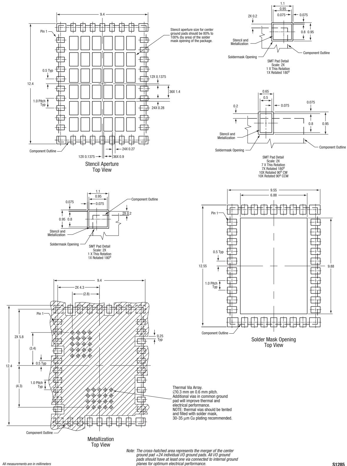
Figure 29. PCB Layout Footprint for the SKY73112-11 9 x 12 mm MCM
