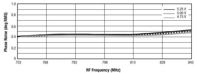
Figure 13. Integrated Phase Noise vs Frequency and Supply Voltage
