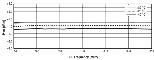
Figure 10. Output Power vs Frequency and Temperature
