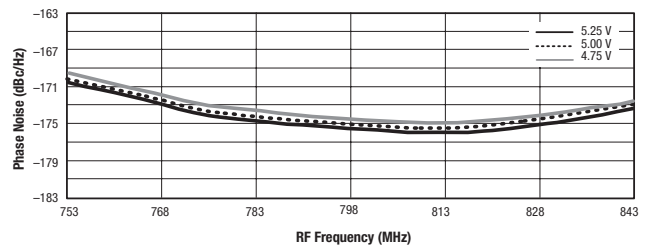
Figure 27. Phase Noise @ 6000 kHz Offset vs Frequency and Supply Voltage
