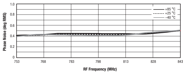
Figure 12. Integrated Phase Noise vs Frequency and Temperature
