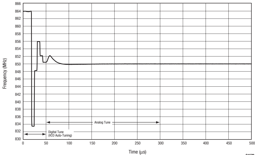
Figure 7. VCO Auto-Tuning @ 850 MHz Frequency Settling
