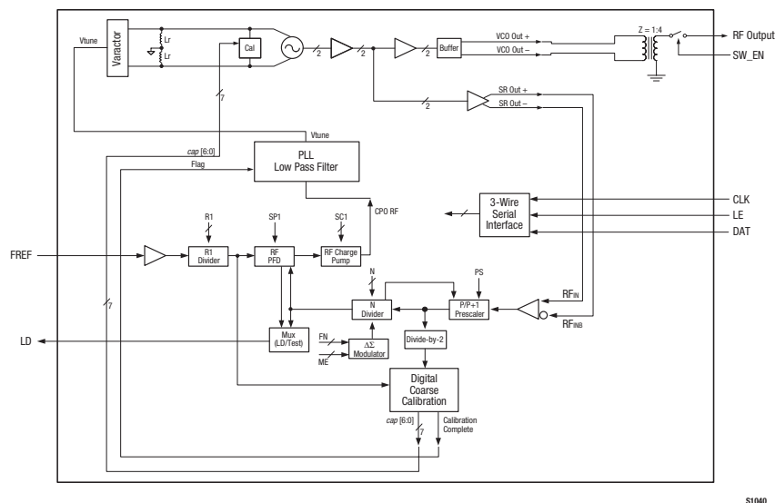
Figure 1. SKY73112-11 Functional Block Diagram
