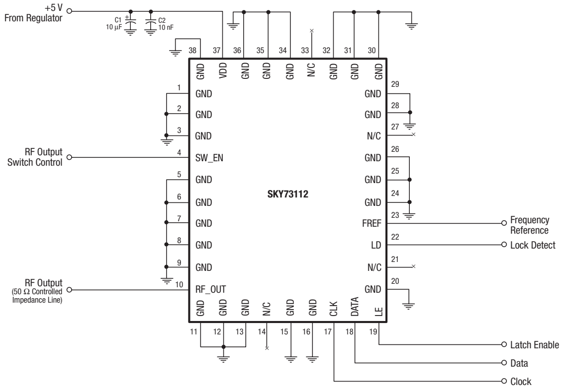
Figure 28. SKY73112-11 Typical Application Schematic
