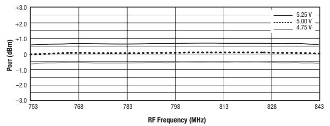
Figure 11. Output Power vs Frequency and Supply Voltage
