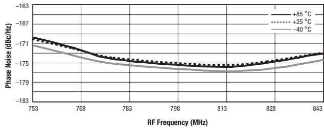
Figure 26. Phase Noise @ 6000 kHz Offset vs Frequency and Temperature
