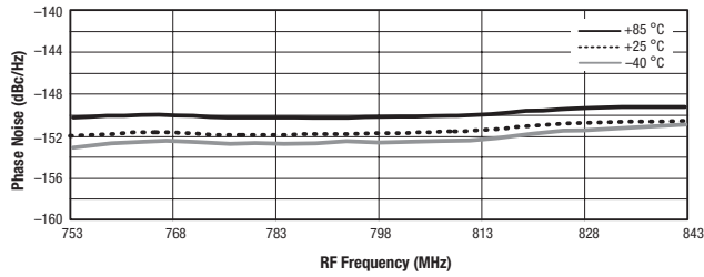
Figure 22. Phase Noise @ 800 kHz Offset vs Frequency and Temperature
