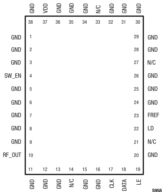
Figure 2. SKY73112-11 Pinout– 38-Pin MCM Package (Top View)
