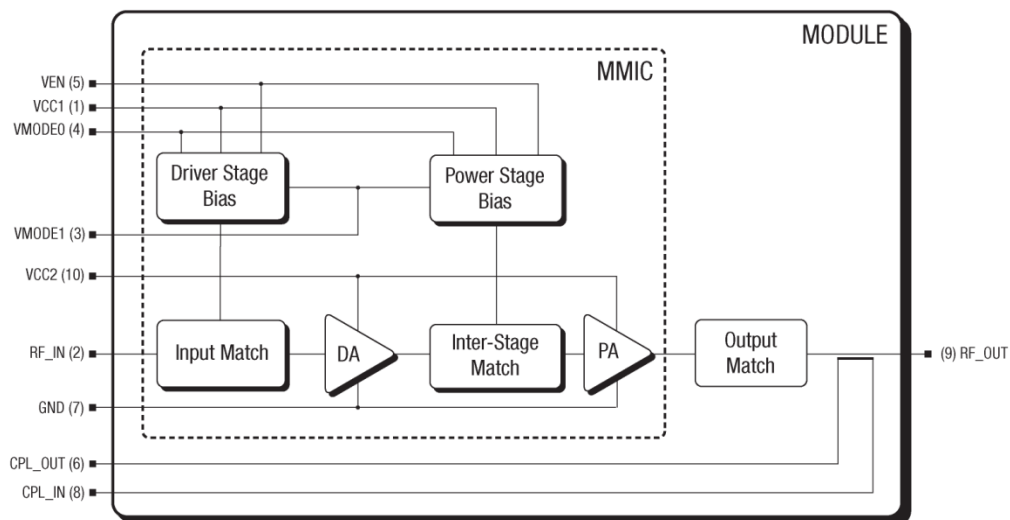
Figure 1. SKY77762 Functional Block Diagram
