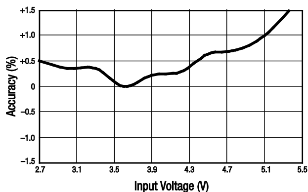
Figure 7. Movie Mode Current Accuracy vs Input Voltage ( I_{MM} = 142\text{ mA} , L = 1\text{ }\mu\text{H} )
