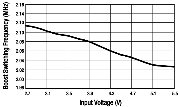
Figure 13. Boost Switching Frequency vs Input Voltage (TA = 25 °C, L = 1 \mu H)
