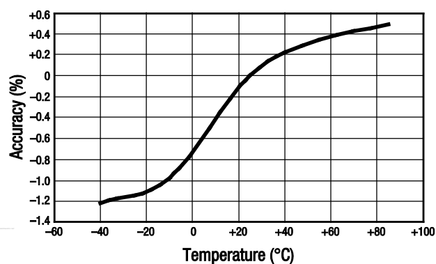
Figure 6. Movie Mode Current Accuracy vs Temperature ( I_{MM} = 142\text{ mA} , V_{IN} = 3.6\text{ V} , L = 1\text{ }\mu\text{H} )
