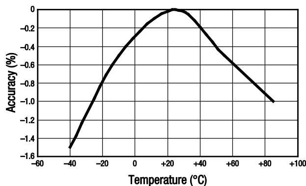
Figure 5. Flash Mode Current Accuracy vs Temperature ( I_{FL} = 1\text{ A} , V_{IN} = 3.6\text{ V} , L = 1\text{ }\mu\text{H} )
