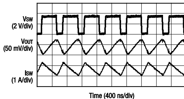
Figure 16. Flash Mode Ripple ( I_{FL} = 1 \text{ A} , C_{OUT} = 2.2 \text{ } \mu\text{F} , V_{IN} = 3.6 \text{ V} , L = 1 \text{ } \mu\text{H} )
