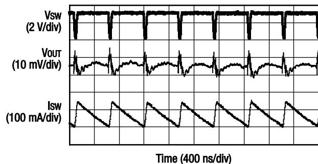
Figure 15. Movie Mode Ripple ( I_{MM} = 142 \text{ mA} , C_{OUT} = 2.2 \text{ } \mu\text{F} , V_{IN} = 3.6 \text{ V} , L = 1 \text{ } \mu\text{H} )
