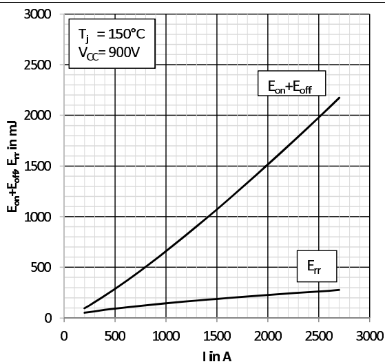
Fig. 3: Typical energy losses E = f(I_C, V_{CC}, T_J)
