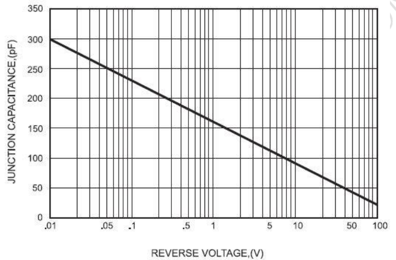
FIG.5-TYPICAL JUNCTION CAPACITANCE
