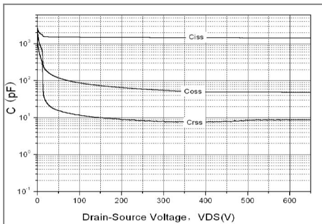
Fig.9. Capacitance characteristics
