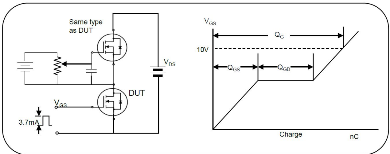
Fig.9. Gate charge test circuit & waveform
