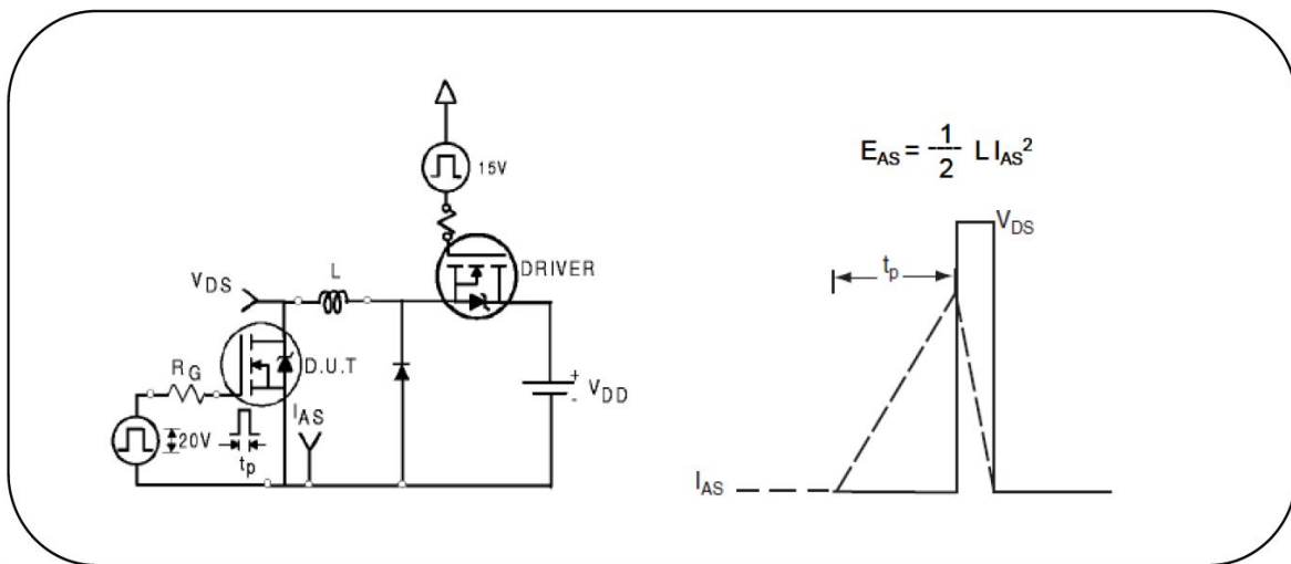
Fig.11. Unclamped inductive switching test circuit & waveform
