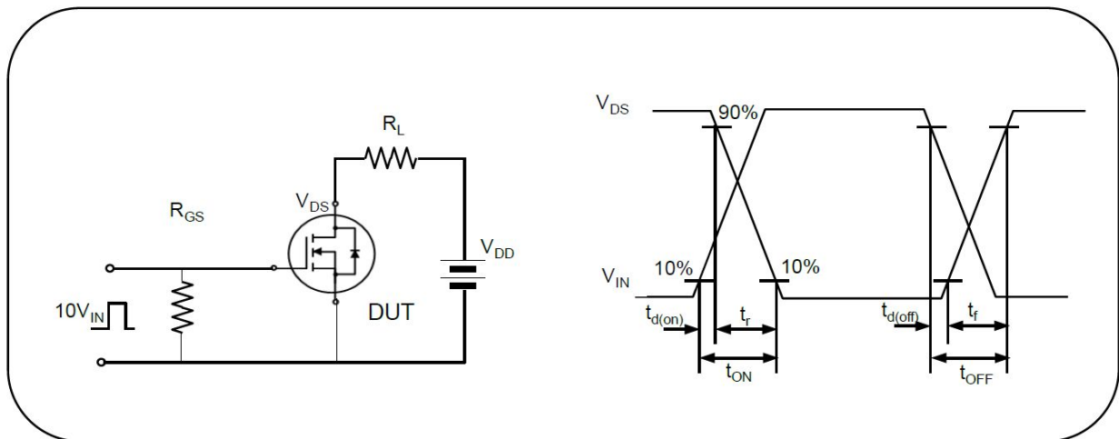
Fig.10. Switching time test circuit & waveform
