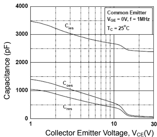
Figure 6. Capacitance Characteristics
