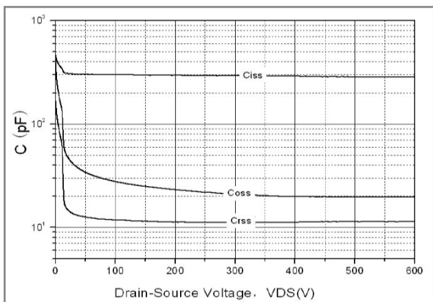
Fig.13. Capacitance characteristics
