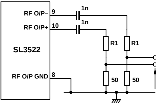
Fig.9 Network for attenuating limited RF output
