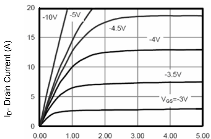
Figure 5 Output Characteristics
