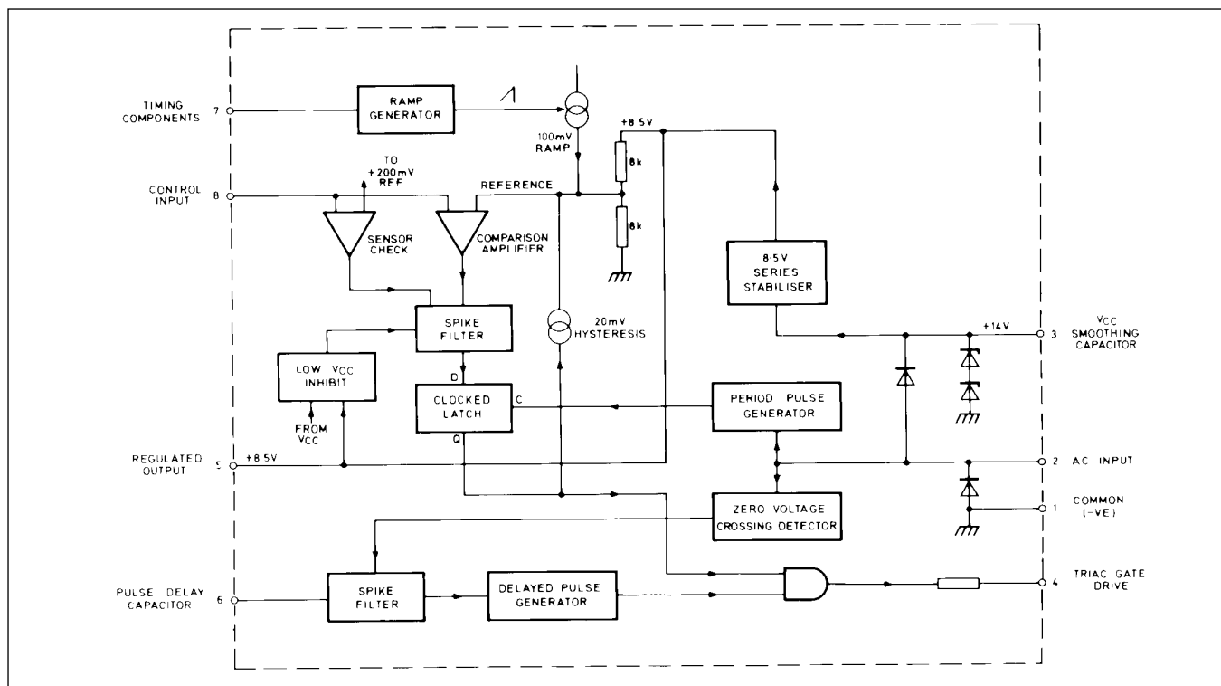
Fig. 2 Block Schematic of SL441C
