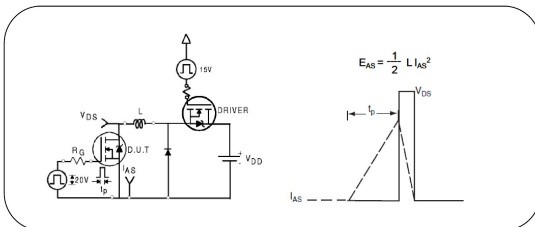
Fig.16. Unclamped inductive switching test circuit & waveform
