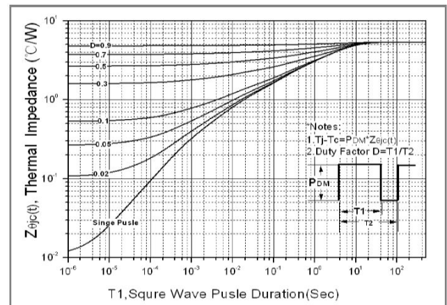
Fig.8. Transient thermal response curve(TO-220FT)
