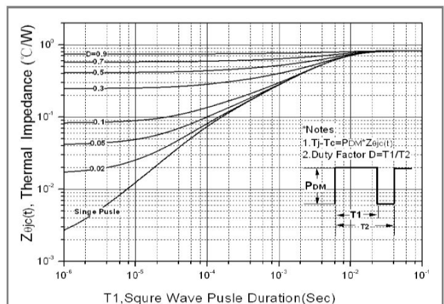
Fig.10. Transient thermal response curve(IPAK)
