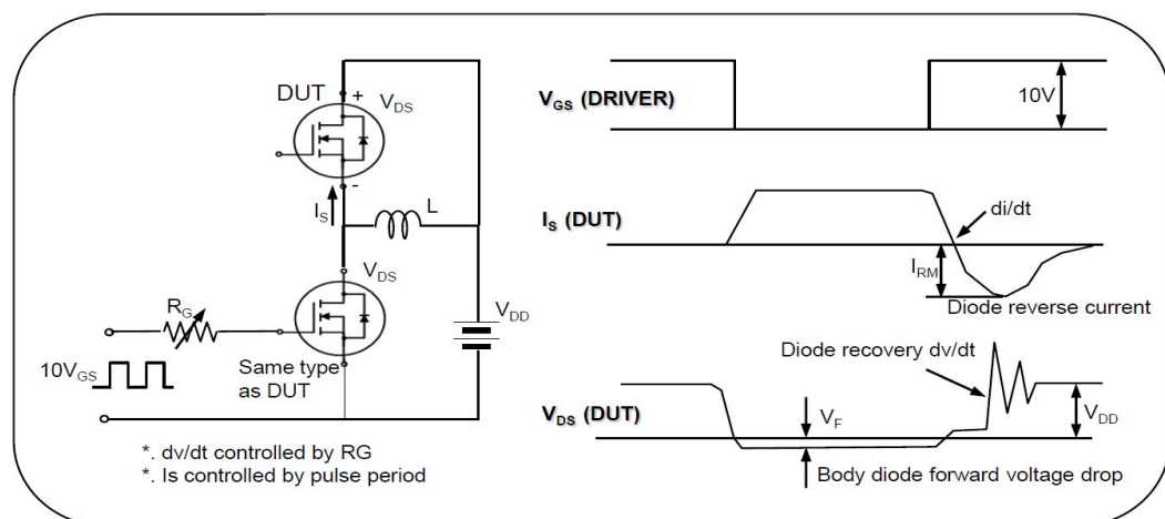
Fig.17. Peak diode recovery dv/dt test circuit & waveform
