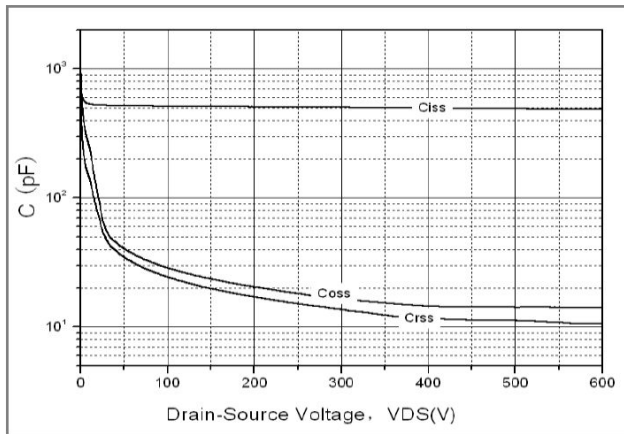
Fig.13. Capacitance characteristics
