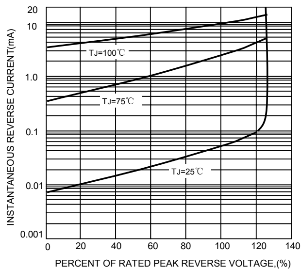
FIG.2-TYPICAL REVER CHARACTERISTICS
