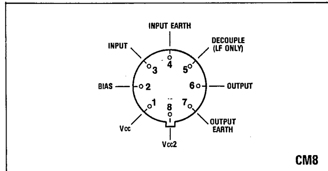
Fig.1 Pin connections
