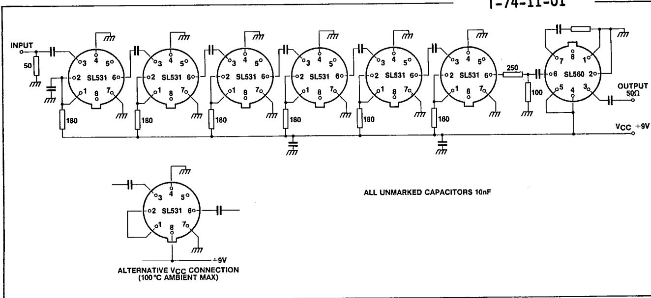
Fig.9 Circuit diagram 6 stage strip
