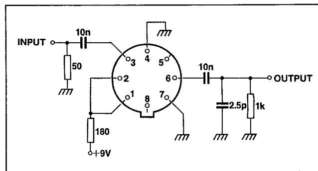
Fig.4 Test circuit
