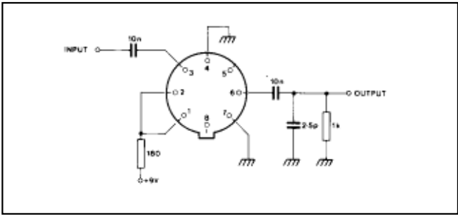
Fig.4 Test circuit
