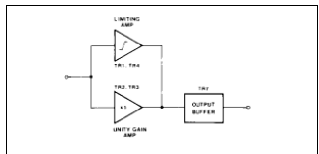
Fig.3 Block diagram
