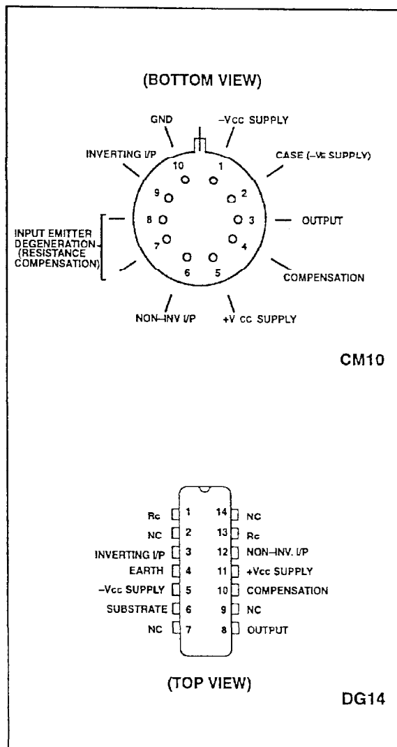
Fig. 1 pin connections
