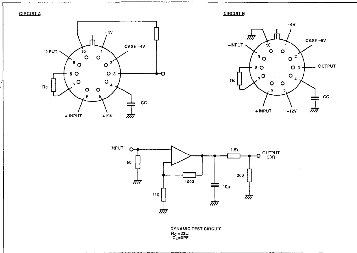
Fig. 8 Test circuit
