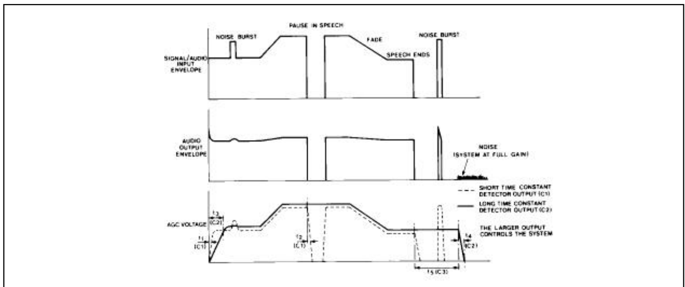
Fig.3 Dynamic response of a system controlled by SL621C AGC generator
