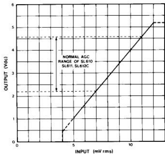
Fig.5 Transfer characteristic of SL621C (typical)
