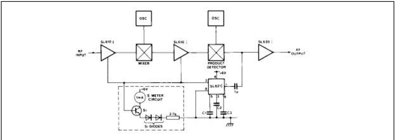
Fig.4 SL621C used to control SSB receiver
