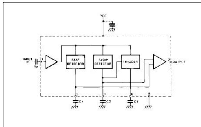
Fig.2 Block diagram
