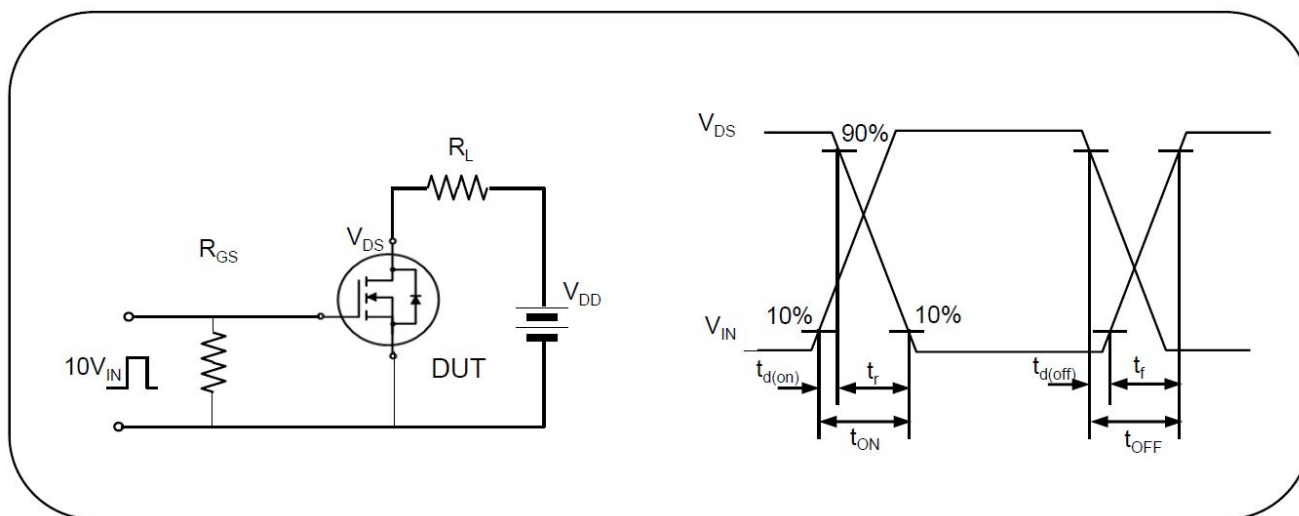
Fig.15. Switching time test circuit & waveform
