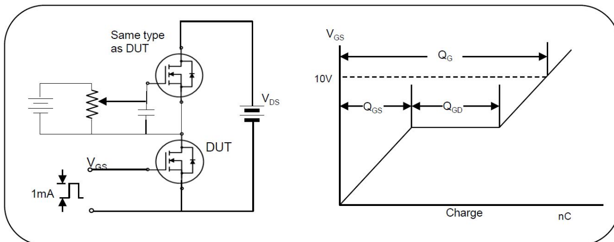
Fig.14. Gate charge test circuit & waveform
