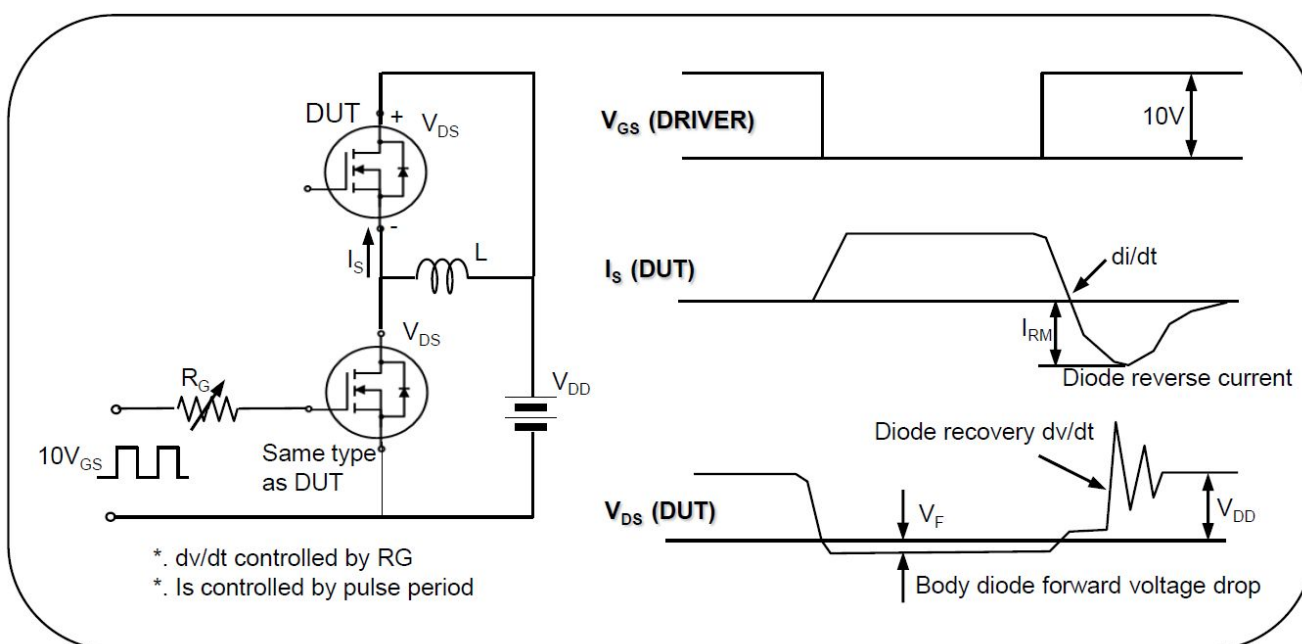
Fig.17. Peak diode recovery dv/dt test circuit & waveform
