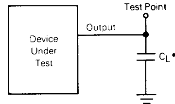
Figure 6. Test Circuit
