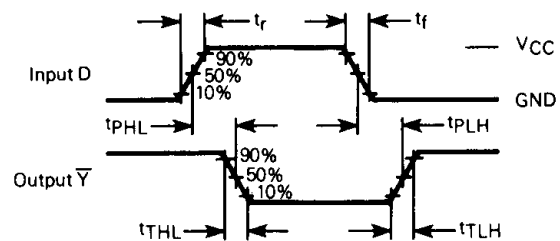
Figure 2. Switching Waveforms
