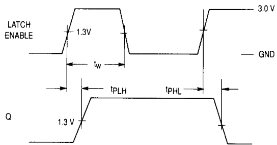
Figure 2. Switching Waveforms
