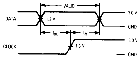
Figure 3. Switching Waveforms
