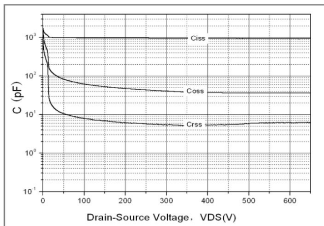
Fig.9. Capacitance characteristics
