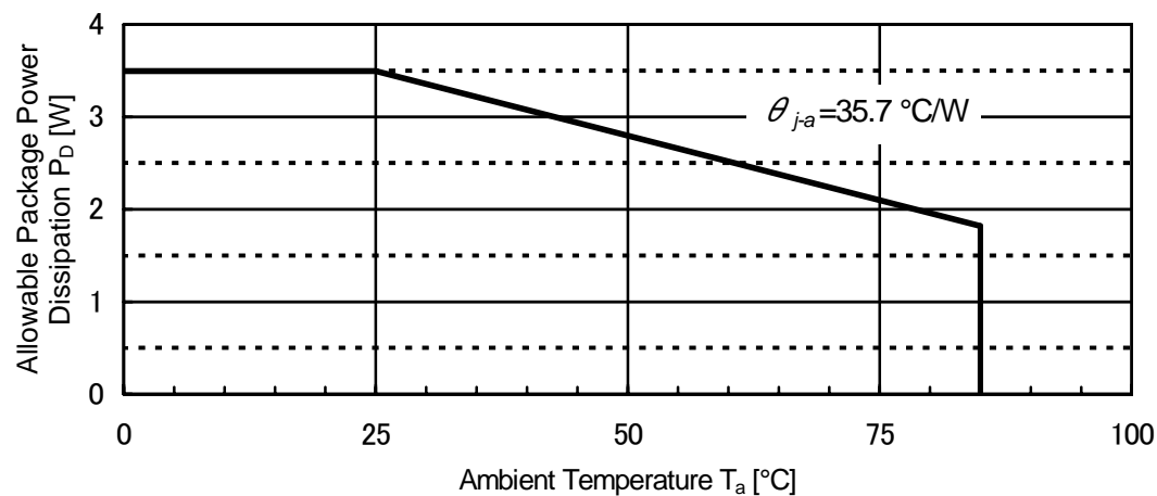
Thermal Ratings
