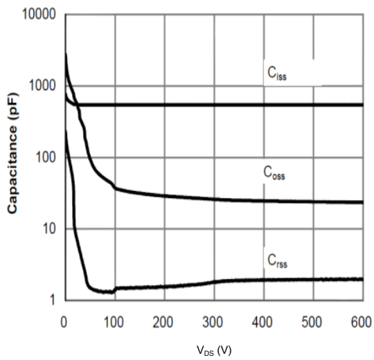
Figure 9: Capacitance Characteristics
