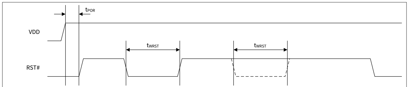
Figure 5 Reset timing
