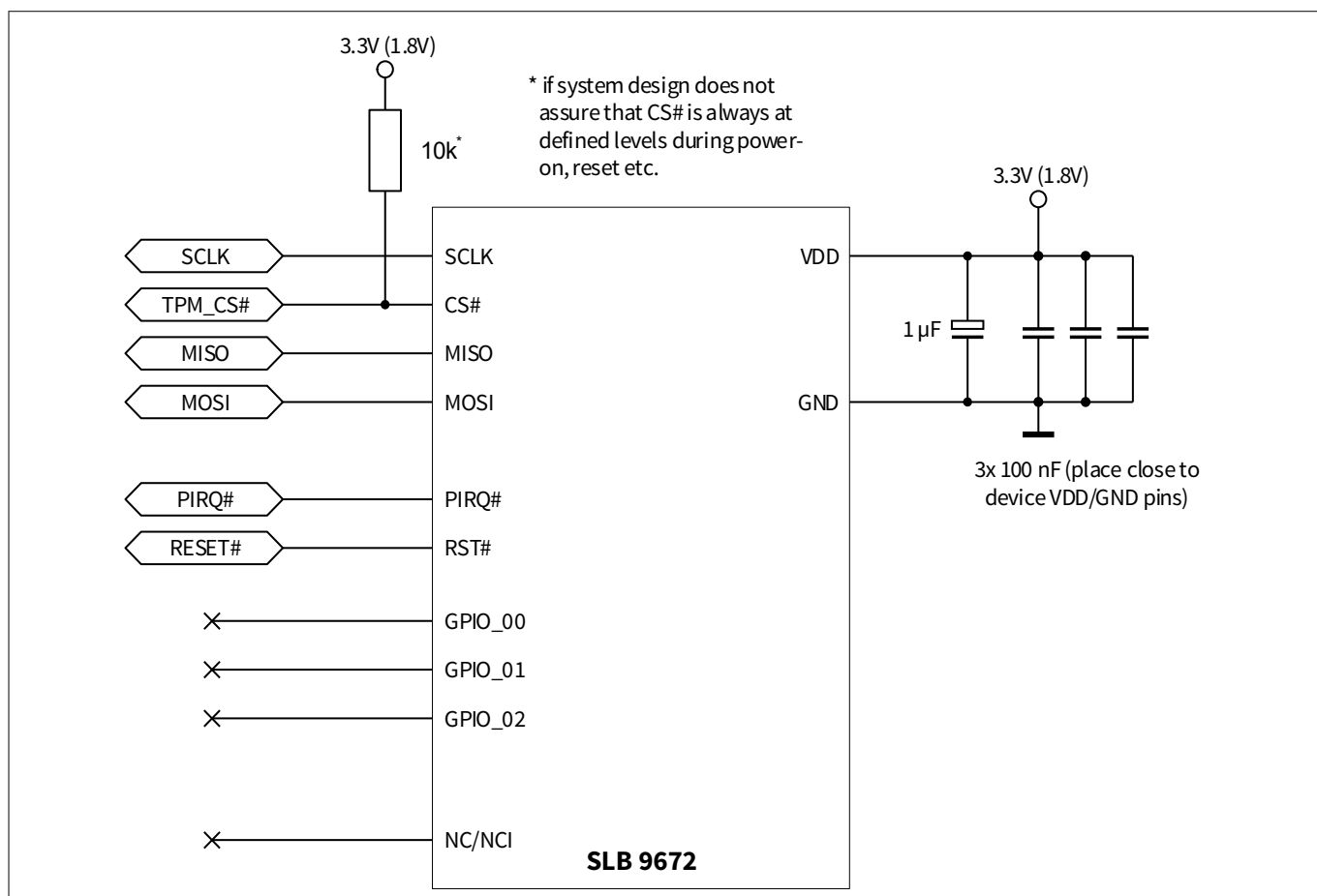
Figure 7 Typical schematic
